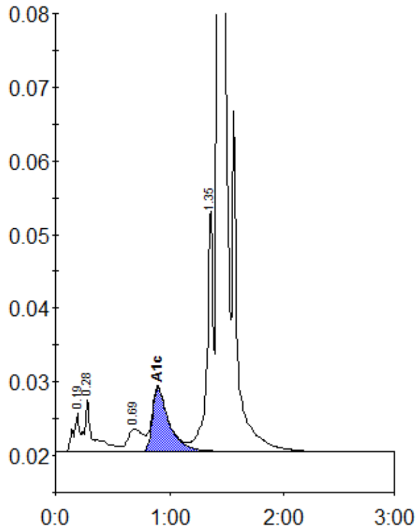
Peak table - ID: 10445947
